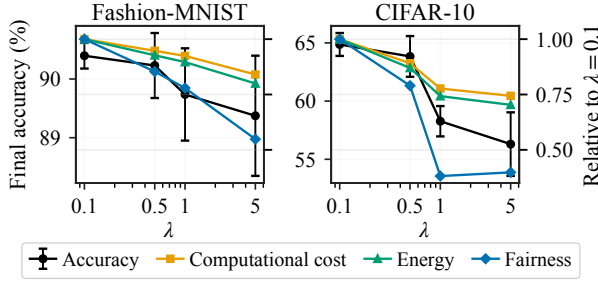
Fig. 4. Sensitivity to the cost trade-off \lambda on Fashion-MNIST (left) and CIFAR-10 (right). The black curve is accuracy, and cost, energy and fairness are normalized to their \lambda = 0.1 values. The CIFAR-10 sweep uses the 100-round protocol of Table III.
